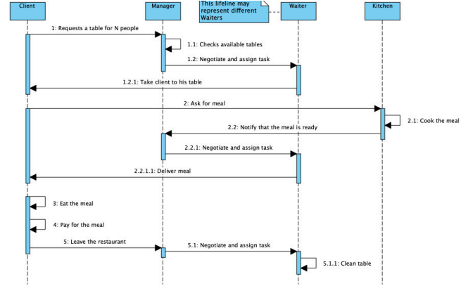
Fig. 6. Multi-agent system - Interaction sequence diagram
