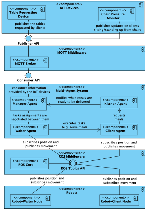
Fig. 4. System architecture
